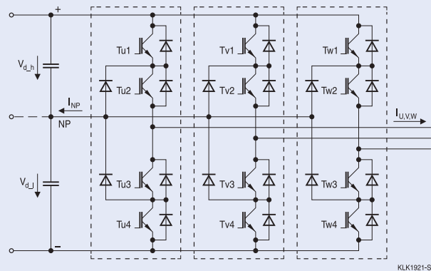
Three-level NPC topology circuit:
