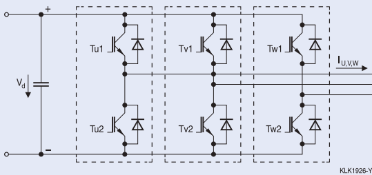
Two-level topology circuit:
